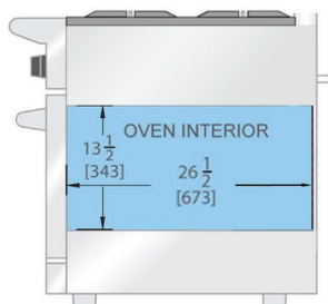
24" and 48" RANGE BASE Larger oven depth accomidates 26" sheet pan front to back.
