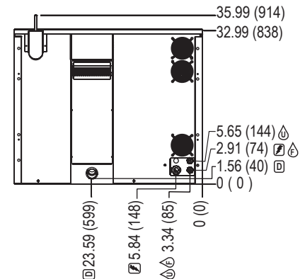
REAR VIEW Single
