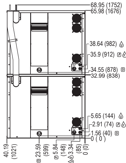
REAR VIEW Double Stack
